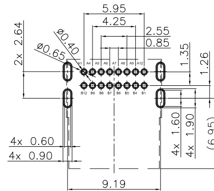
RECOMMENDED PCB LAYOUT(TOP) TOLERANCES:±0.05MM
